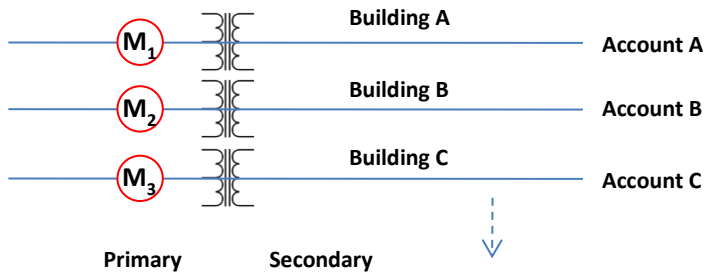
Diagram 5: Primary Metering, Non-Totalized, 2 or More Metering Points
